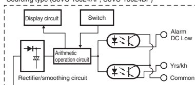
Sourcing type (S8VS-18024AP, S8VS-18024BP)
