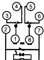
LED indicator and Varistor type (AC coil) MK2PNV-I, -S
