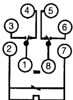
Varistor type (AC coil) MK2PV-I, -S
