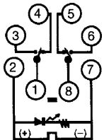
LED indicator type (DC coil) MK2PN-I, -S
