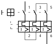
1-pole
