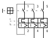
2-pole
