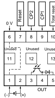
H7CX-ASD/-A4SD 1-stage Transistor Output
