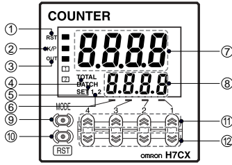
Front view of 4-digit model
