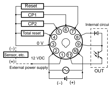
H7CX-A11S/-A114S/-A11SD1 1-stage Transistor Output
