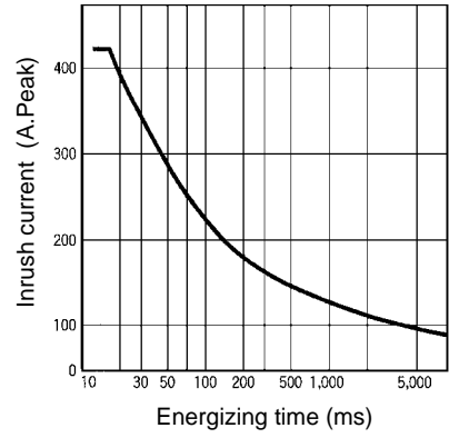
G3PX-260E Models
