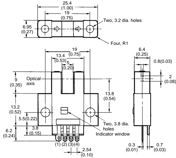
Terminal Arrangement
