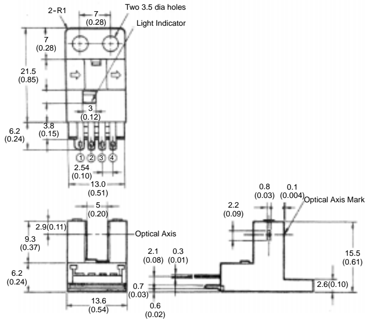
Terminal Arrangement
