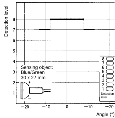
E3MC-(M)Aj j (X Direction)
