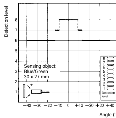
E3MC-(M)Xj j (X Direction)
