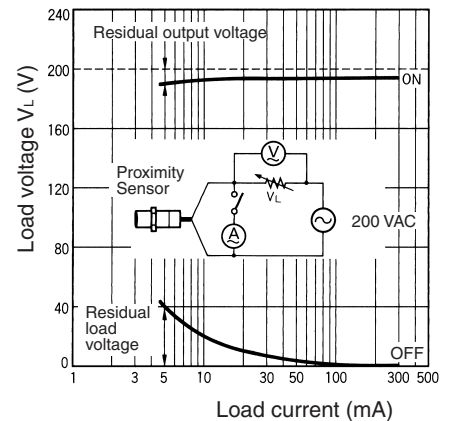
200 VAC
